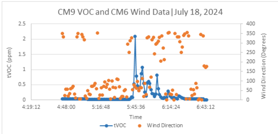
FIGURE 1-2 CM9 tVOC AND CM6 WIND DIRECTION | July 18, 2024, 7:10 A.M. – 9:10 A.M.
