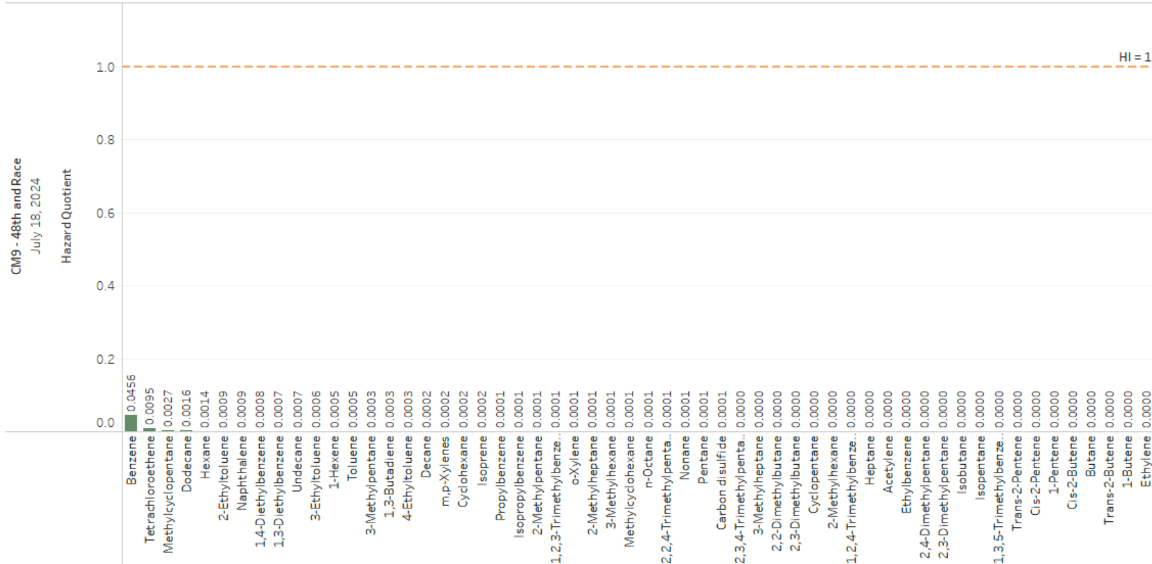
FIGURE 1-4 COMPOUND-SPECIFIC HAZARD QUOTIENTS FOR VOCS DETECTED IN THE JULY 18, 2024, SENSOR-TRIGGERED EVENT SAMPLE AT CM9 – 48 th AND RACE LOCATION
