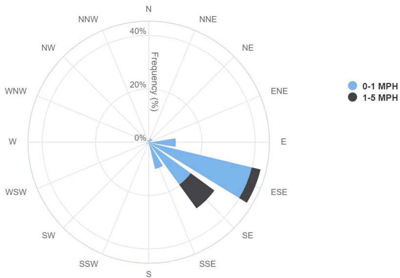
FIGURE 1-3 CM5 WIND ROSE | September 23, 2024, 2:30 A.M. – 4:30 A.M.
