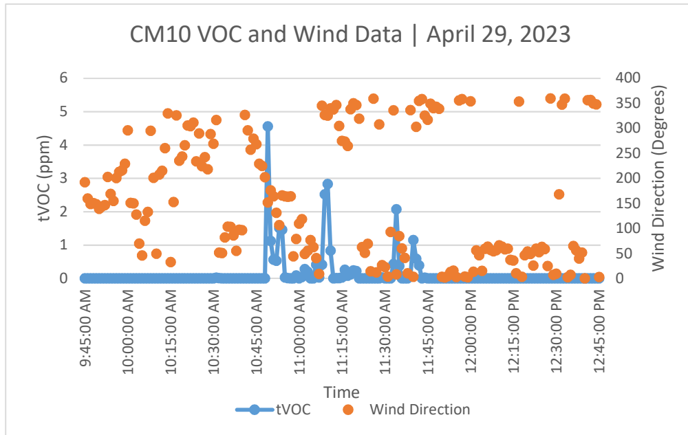
FIGURE 1-2 CM10 VOC AND WIND DIRECTION | APRIL 29, 2023, 9:45 A.M. – 12:45 P.M.
